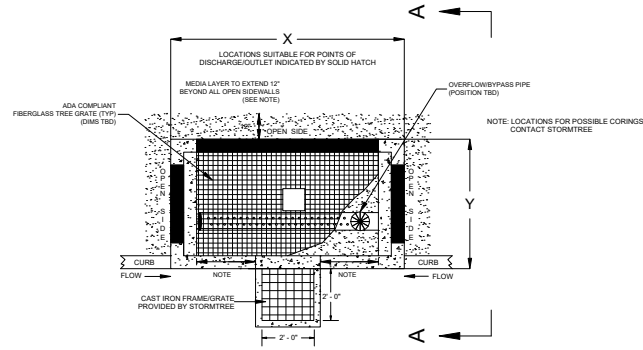
PLAN VIEW NOT TO SCALE
